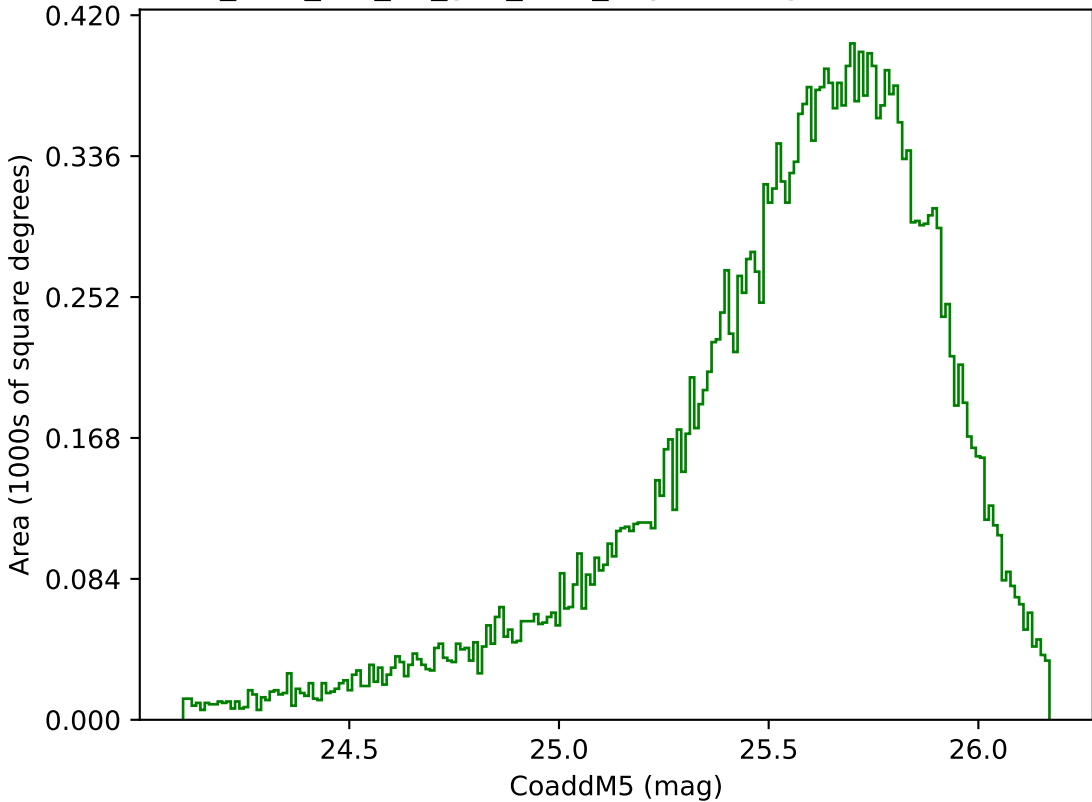
too_elab_r64_d2_griz_v3.4_10yrs Yr 1 g band: CoaddM5
