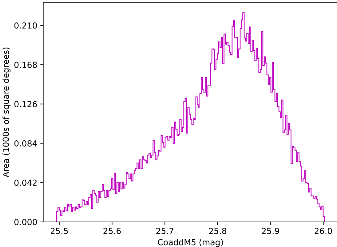
too_elab_r64_d2_griz_v3.4_10yrs WFD z band: CoaddM5
