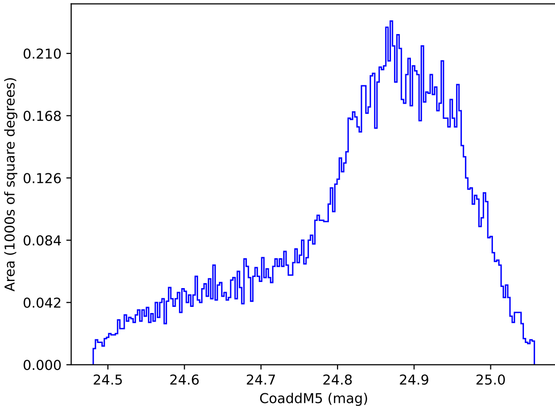
too_elab_r64_d2_griz_v3.4_10yrs WFD y band: CoaddM5
