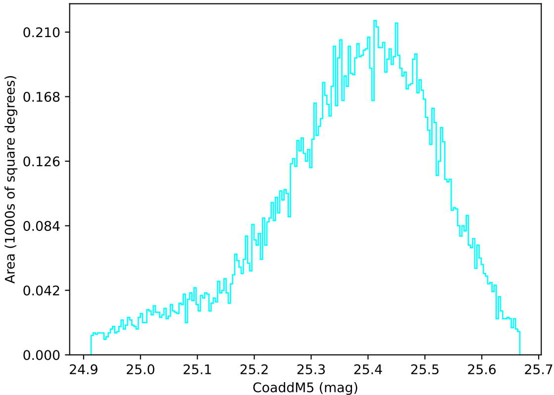
too_elab_r64_d2_griz_v3.4_10yrs WFD u band: CoaddM5
