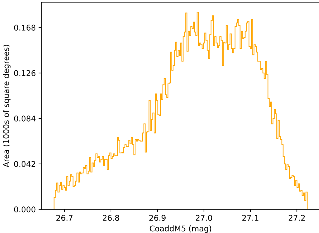
too_elab_r64_d2_griz_v3.4_10yrs WFD r band: CoaddM5
