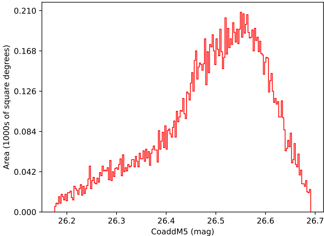
too_elab_r64_d2_griz_v3.4_10yrs WFD i band: CoaddM5
