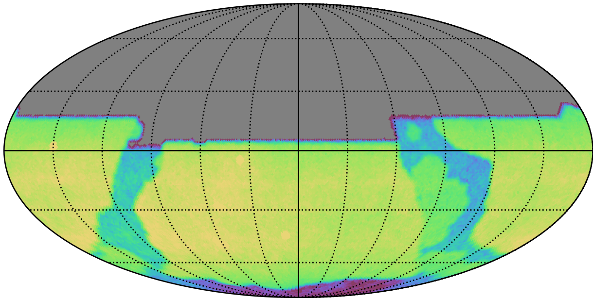
too_elab_r64_d2_griz_v3.4_10yrs All sky y band: CoaddM5
