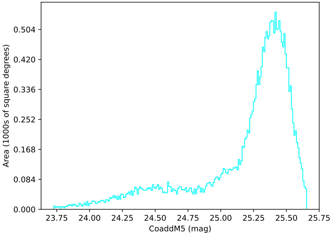
too_elab_r64_d2_griz_v3.4_10yrs All sky u band: CoaddM5
