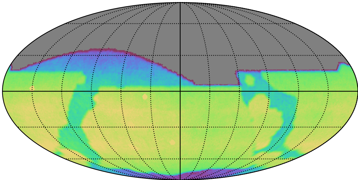
too_elab_r64_d2_griz_v3.4_10yrs All sky r band: CoaddM5
