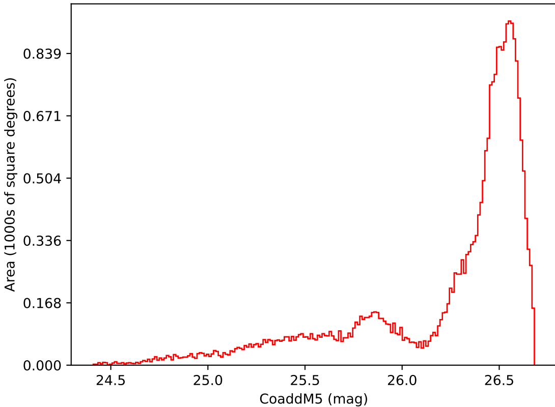
too_elab_r64_d2_griz_v3.4_10yrs All sky i band: CoaddM5
