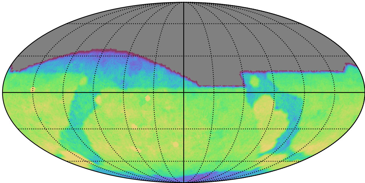
too_elab_r64_d2_griz_v3.4_10yrs All sky g band: CoaddM5
