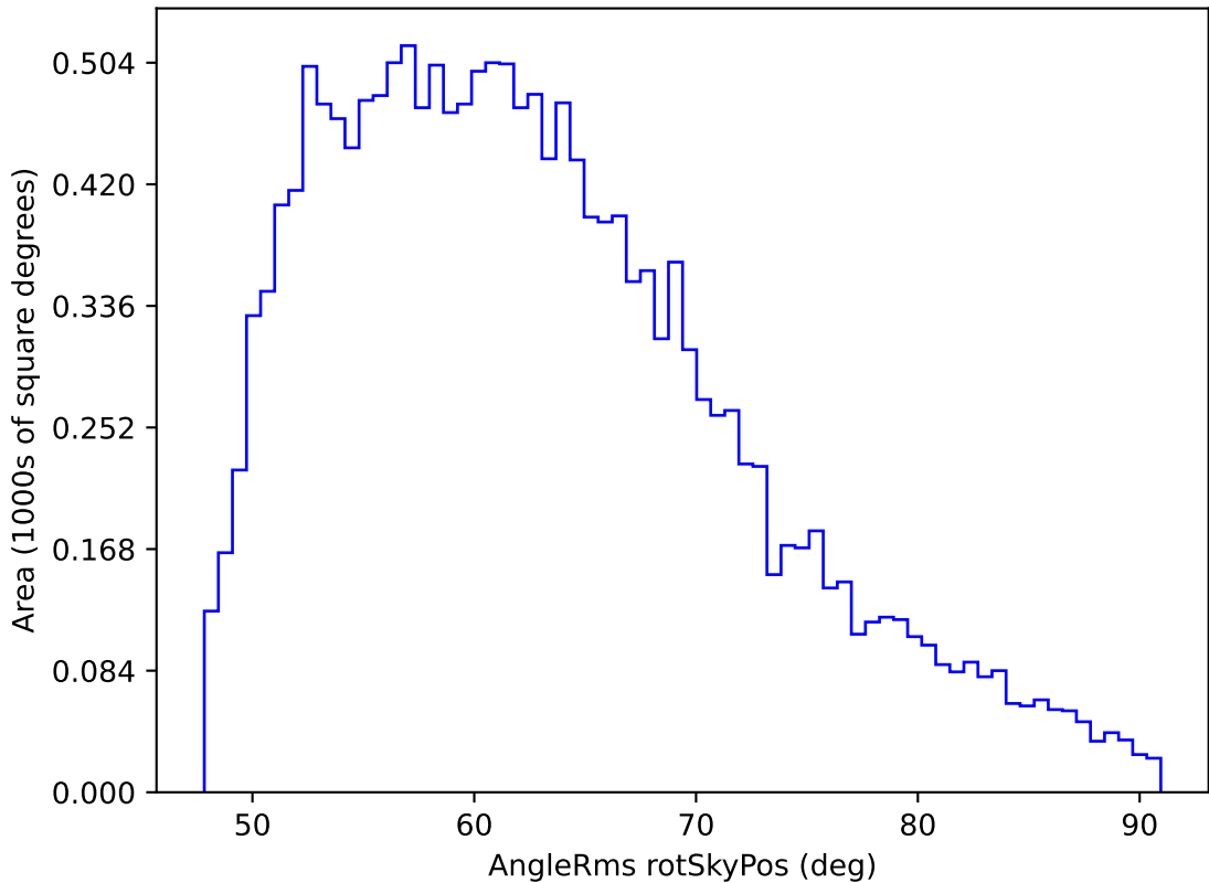
too_elab_r64_d2_griz_v3.4_10yrs WFD y band: AngleRms rotSkyPos
