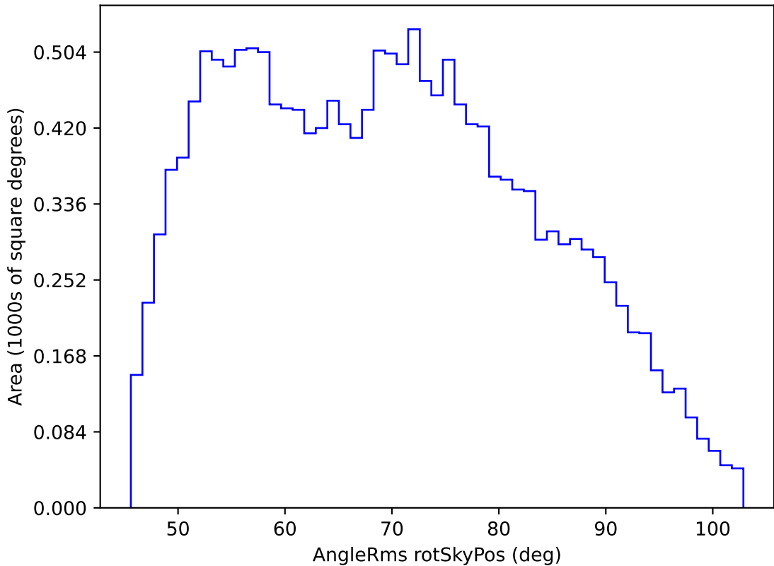
too_elab_r64_d2_griz_v3.4_10yrs WFD g band: AngleRms rotSkyPos
