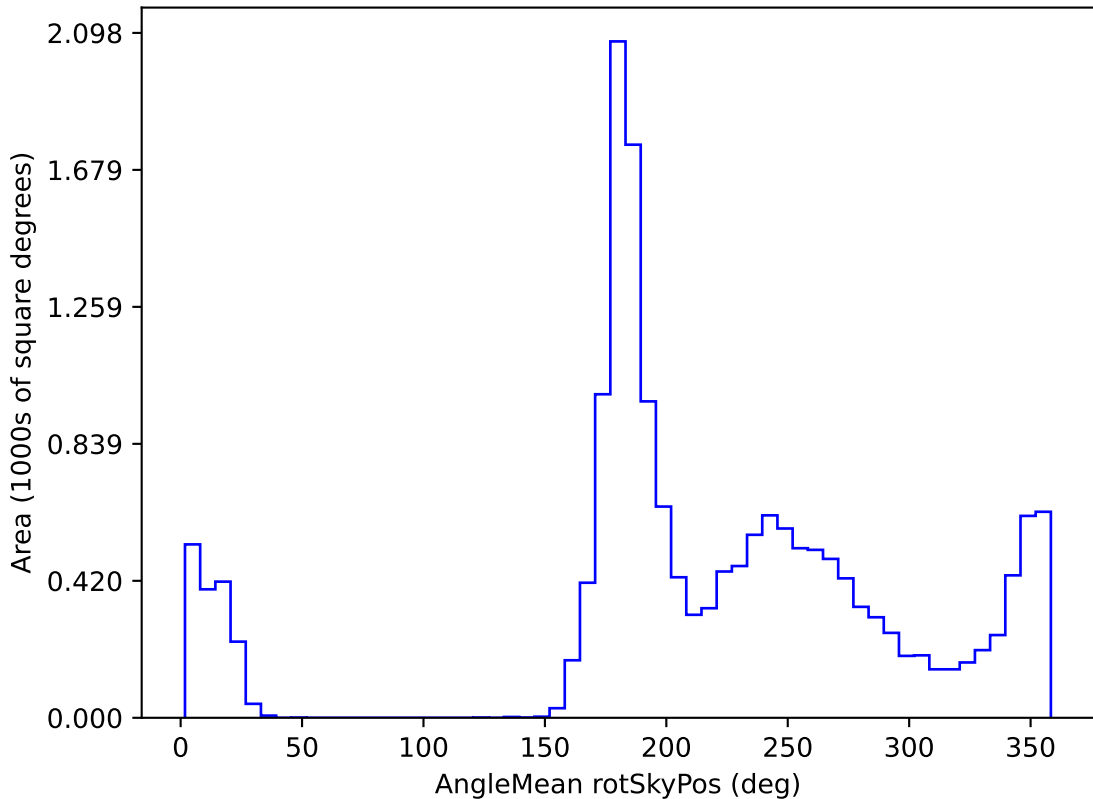
too_elab_r64_d2_griz_v3.4_10yrs WFD i band: AngleMean rotSkyPos
