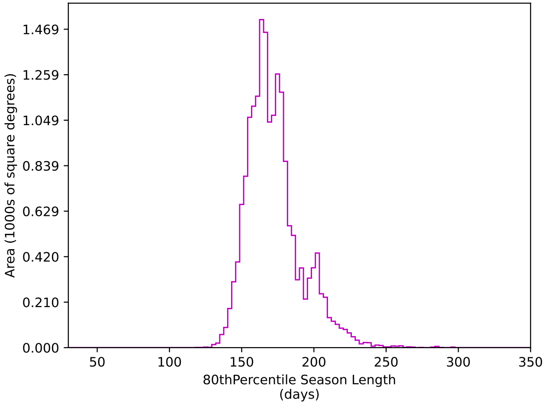
too_elab_r64_d2_griz_v3.4_10yrs WFD z band: 80thPercentile Season Length
