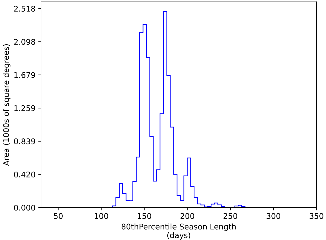
too_elab_r64_d2_griz_v3.4_10yrs WFD y band: 80thPercentile Season Length
