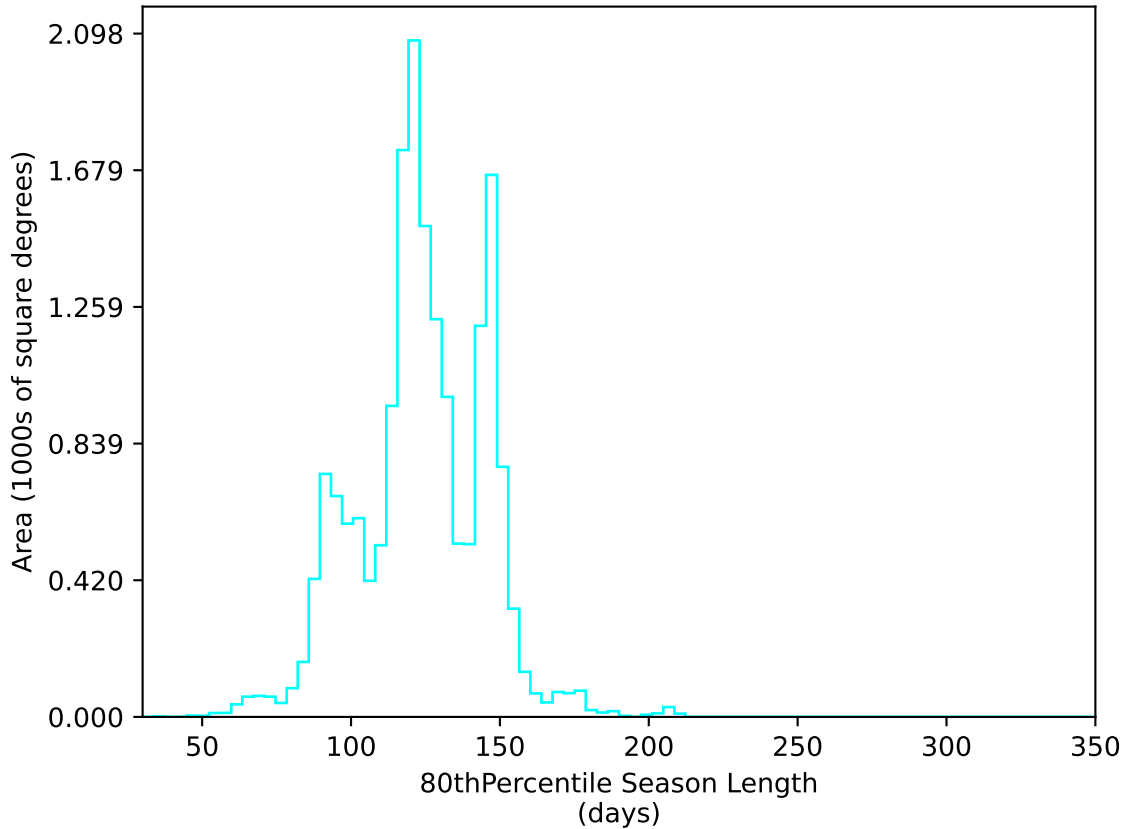
too_elab_r64_d2_griz_v3.4_10yrs WFD u band: 80thPercentile Season Length
