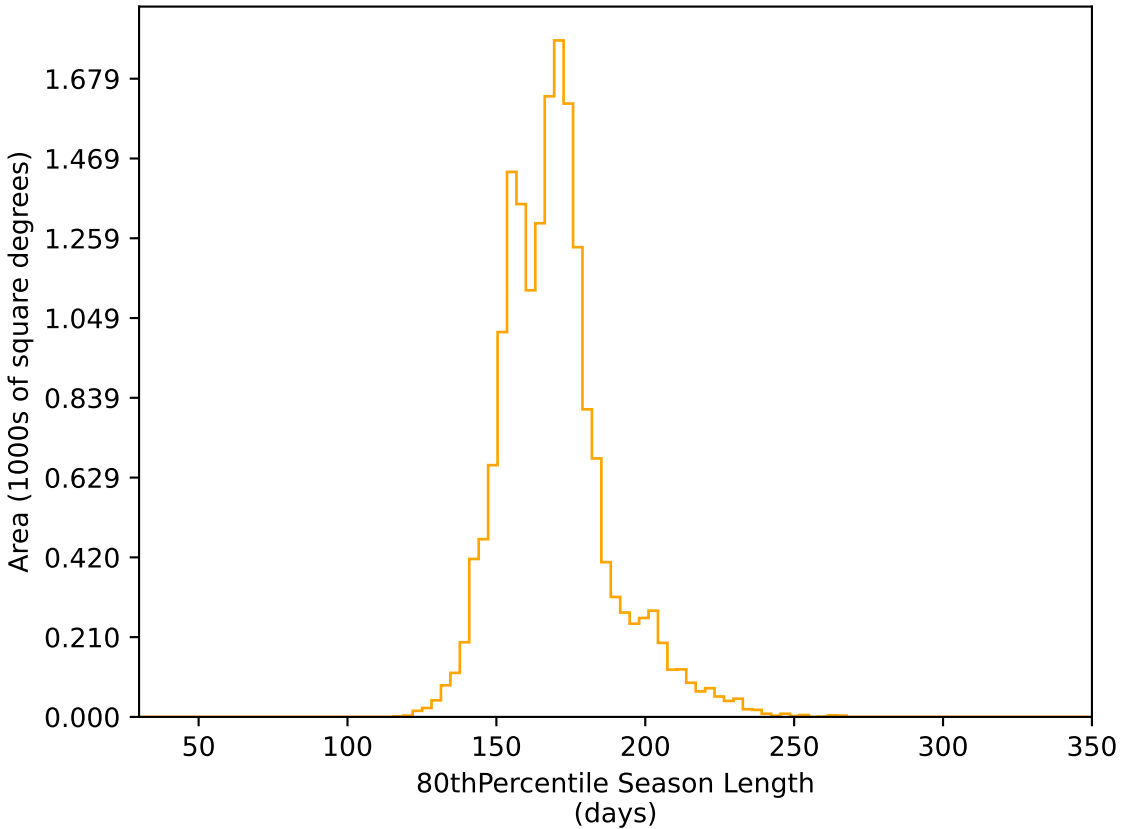
too_elab_r64_d2_griz_v3.4_10yrs WFD r band: 80thPercentile Season Length
