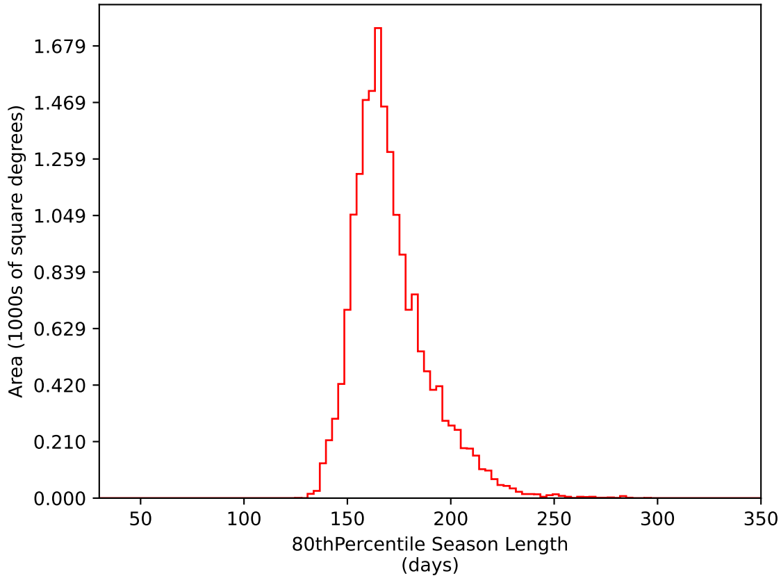
too_elab_r64_d2_griz_v3.4_10yrs WFD i band: 80thPercentile Season Length
