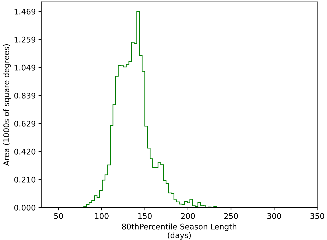
too_elab_r64_d2_griz_v3.4_10yrs WFD g band: 80thPercentile Season Length
