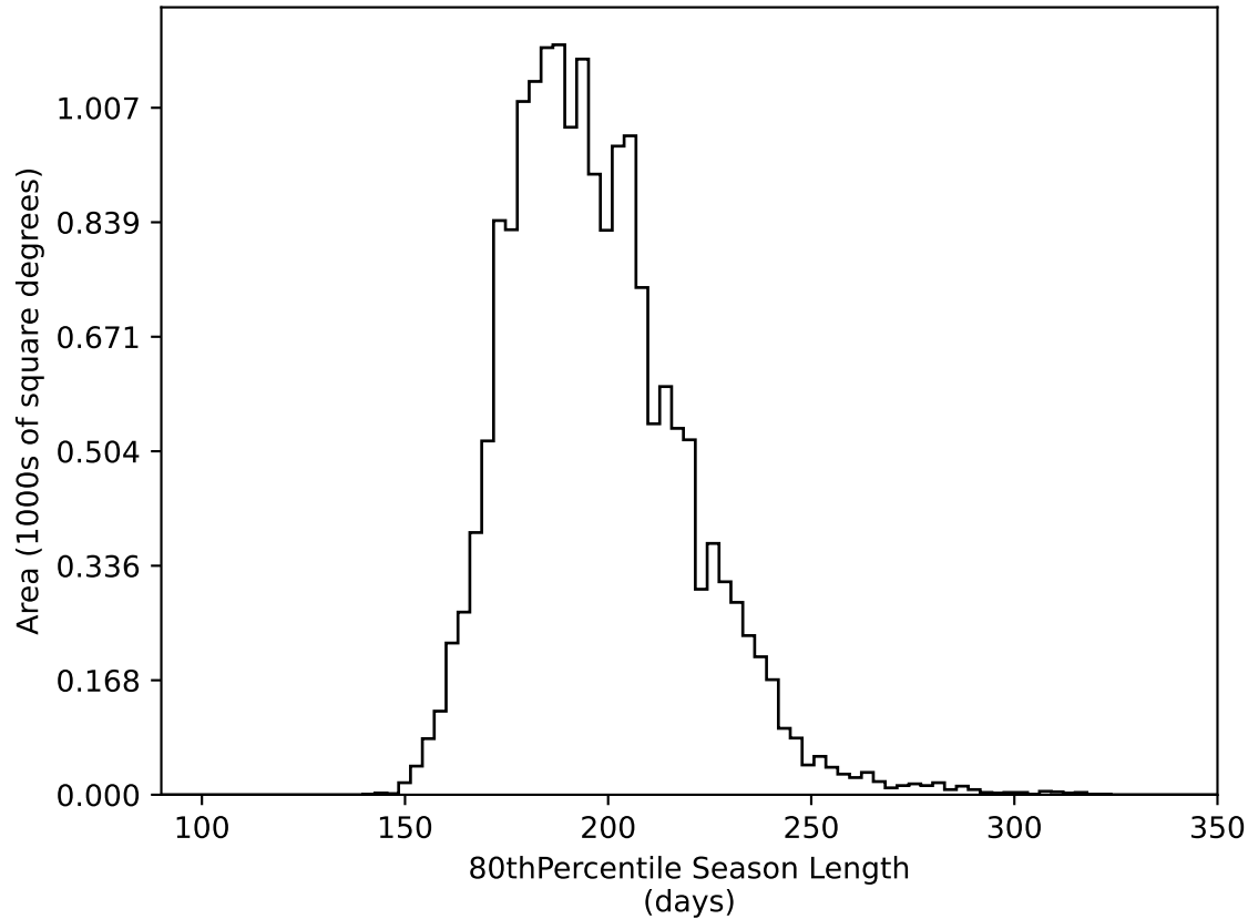
too_elab_r64_d2_griz_v3.4_10yrs WFD all bands: 80thPercentile Season Length
