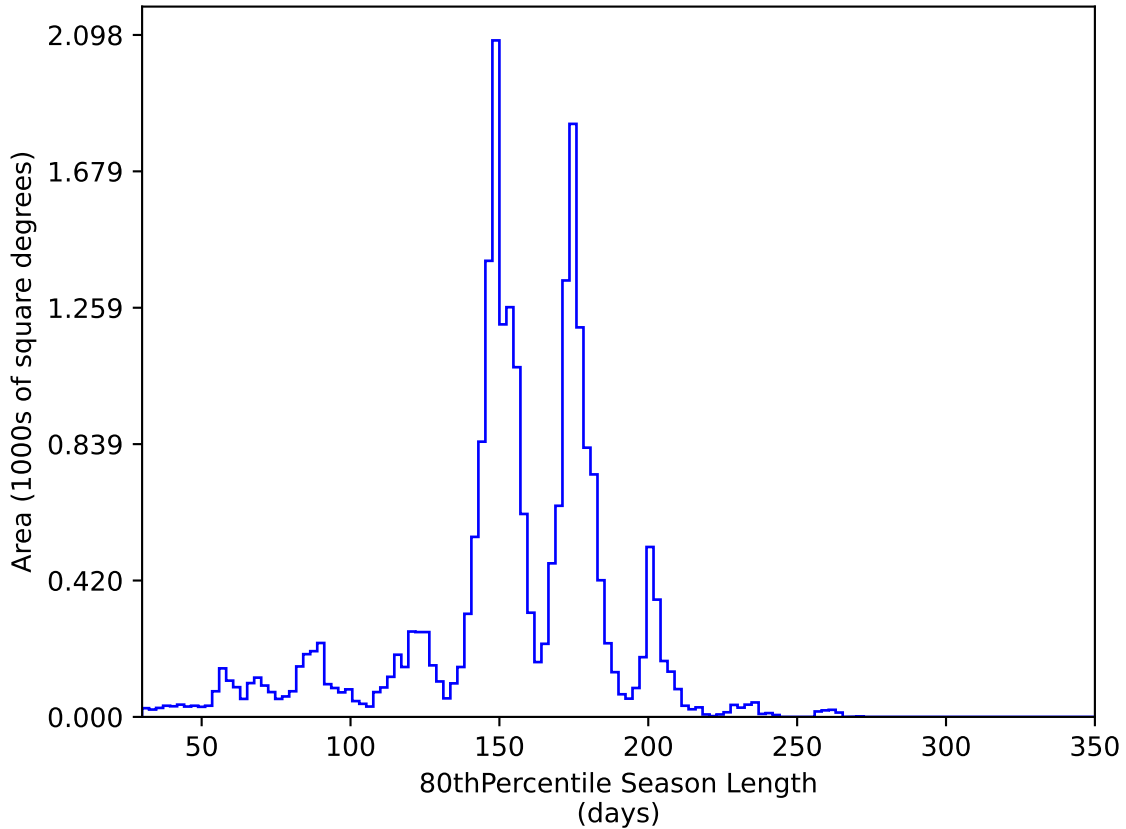
too_elab_r64_d2_griz_v3.4_10yrs All sky y band: 80thPercentile Season Length
