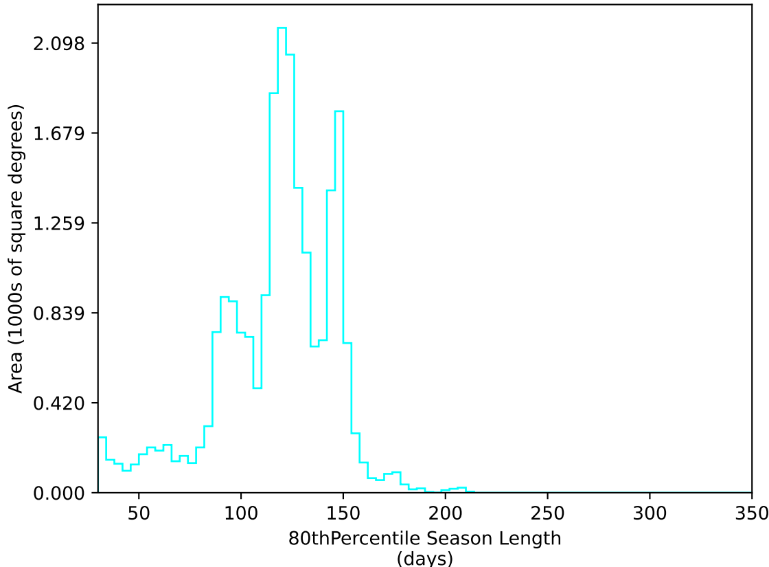
too_elab_r64_d2_griz_v3.4_10yrs All sky u band: 80thPercentile Season Length
