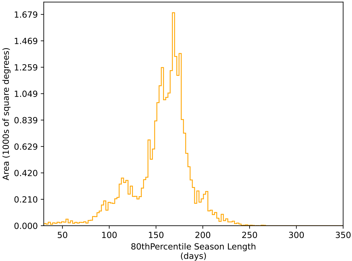
too_elab_r64_d2_griz_v3.4_10yrs All sky r band: 80thPercentile Season Length
