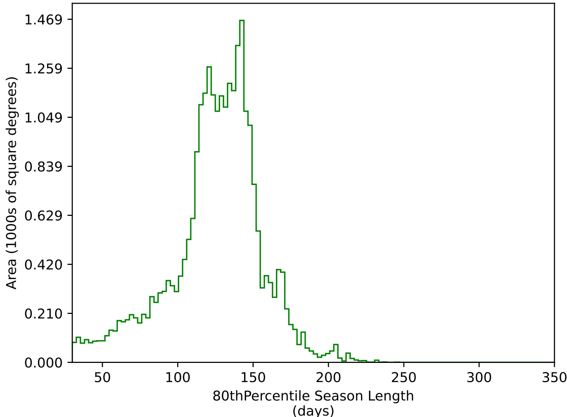
too_elab_r64_d2_griz_v3.4_10yrs All sky g band: 80thPercentile Season Length
