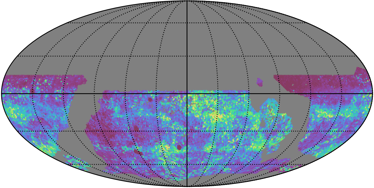
too_elab_r64_d2_griz_v3.4_10yrs WFD zy bands: 75th Percentile Intranight Timespan
