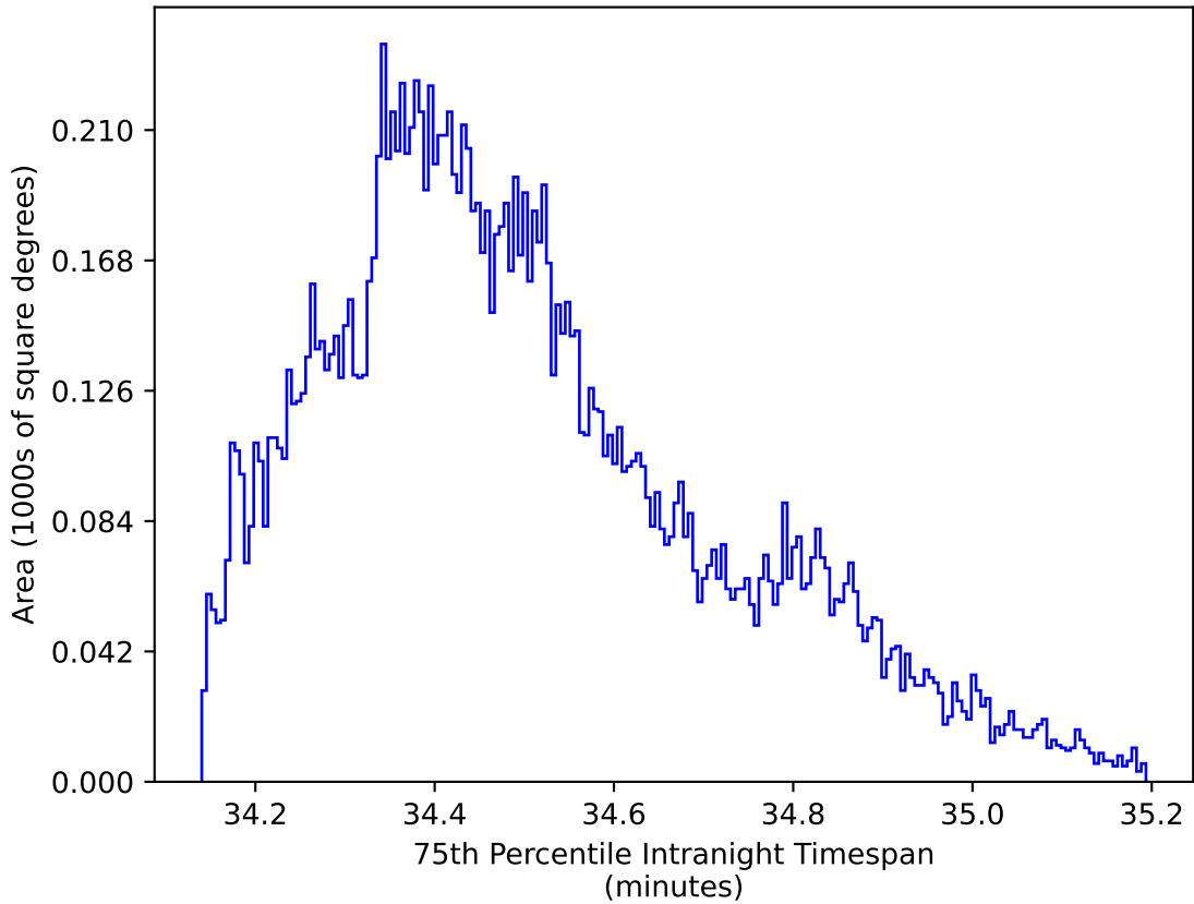
too_elab_r64_d2_griz_v3.4_10yrs WFD zy bands: 75th Percentile Intranight Timespan
