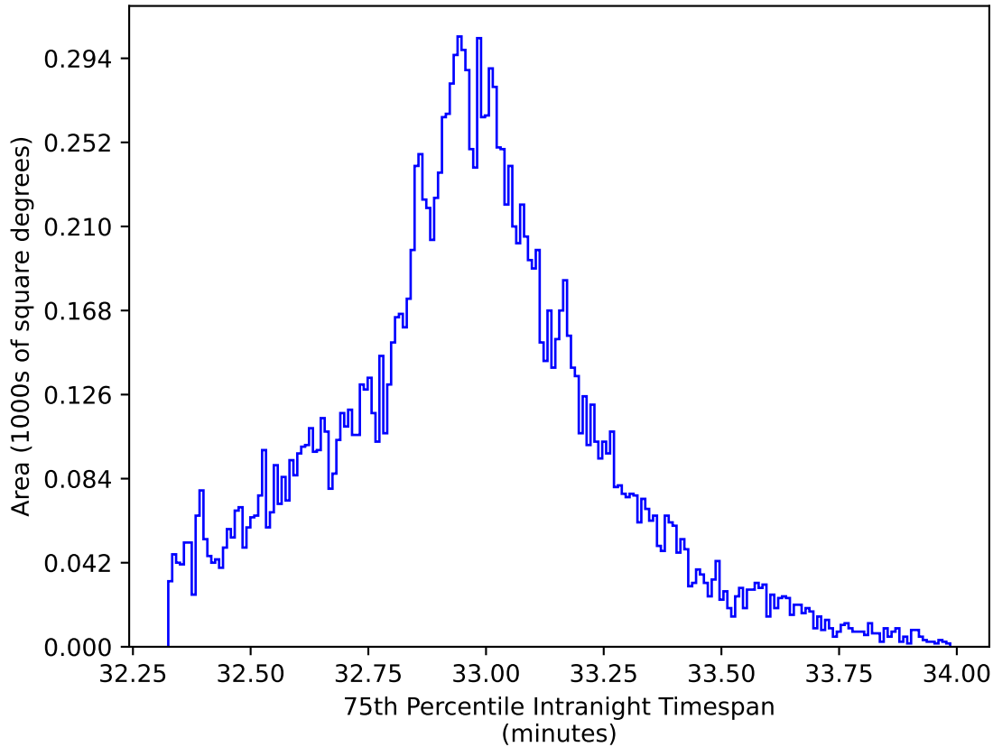
too_elab_r64_d2_griz_v3.4_10yrs WFD y band: 75th Percentile Intranight Timespan
