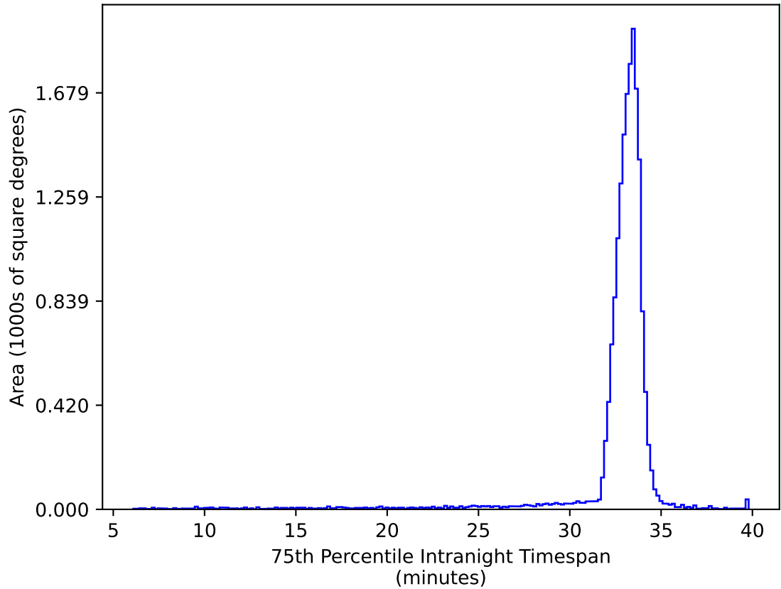
too_elab_r64_d2_griz_v3.4_10yrs WFD ug bands: 75th Percentile Intranight Timespan
