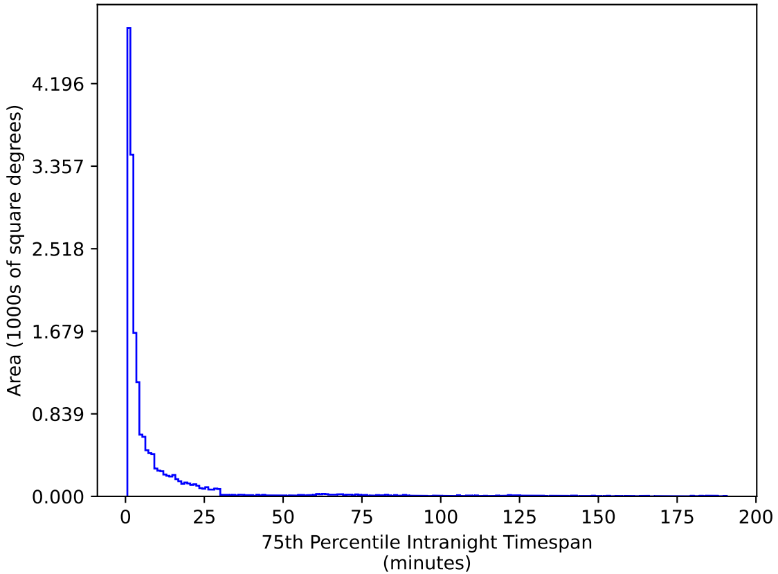
too_elab_r64_d2_griz_v3.4_10yrs WFD u band: 75th Percentile Intranight Timespan
