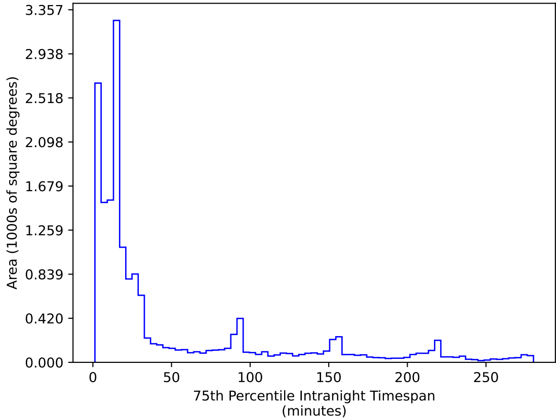
too_elab_r64_d2_griz_v3.4_10yrs WFD r band: 75th Percentile Intranight Timespan
