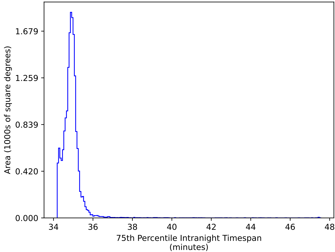
too_elab_r64_d2_griz_v3.4_10yrs WFD iz bands: 75th Percentile Intranight Timespan
