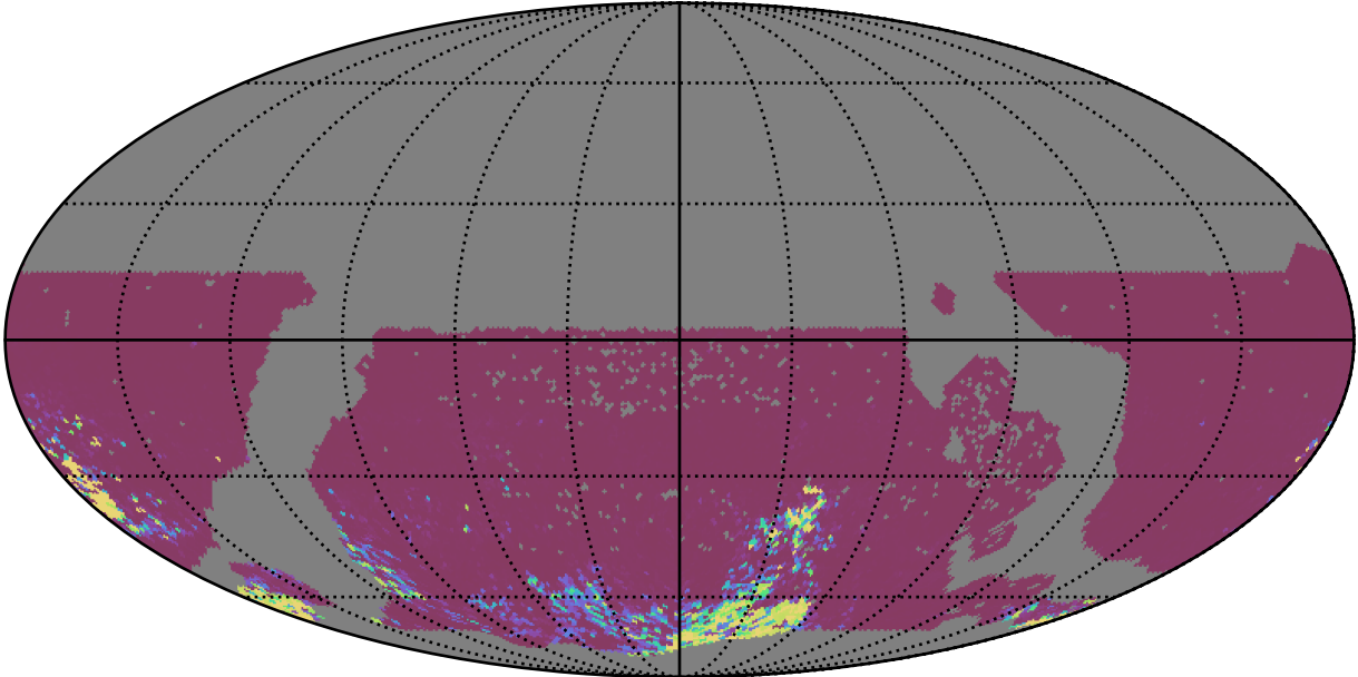
too_elab_r64_d2_griz_v3.4_10yrs WFD gr bands: 75th Percentile Intranight Timespan
