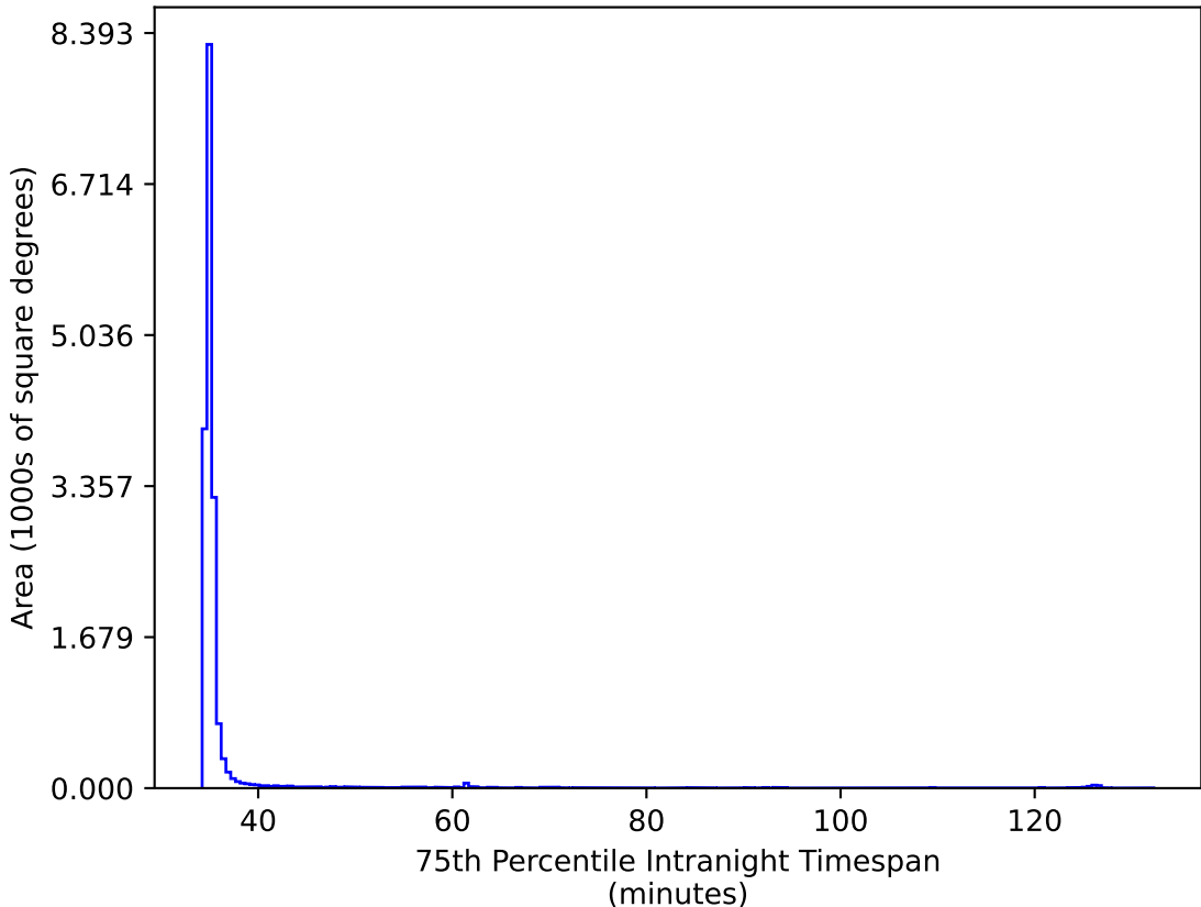
too_elab_r64_d2_griz_v3.4_10yrs WFD gr bands: 75th Percentile Intranight Timespan
