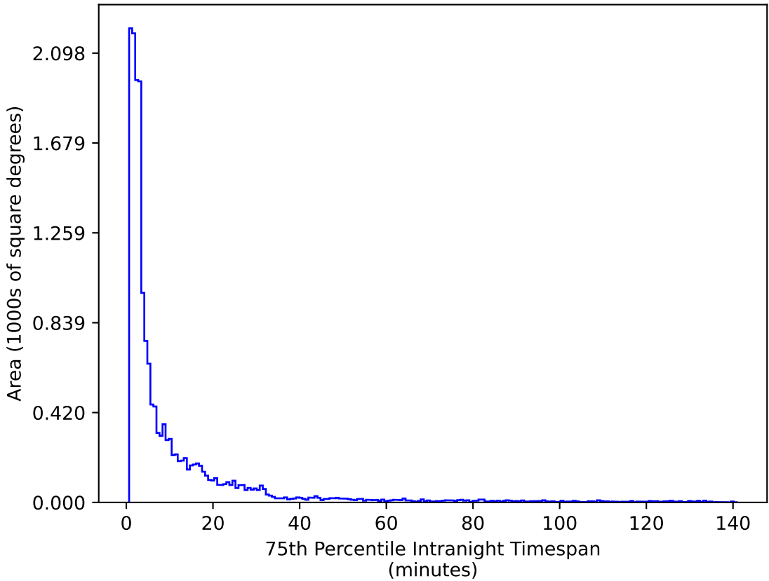
too_elab_r64_d2_griz_v3.4_10yrs WFD g band: 75th Percentile Intranight Timespan
