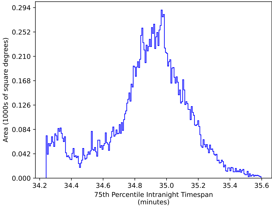
too_elab_r64_d2_griz_v3.4_10yrs WFD all bands: 75th Percentile Intranight Timespan
