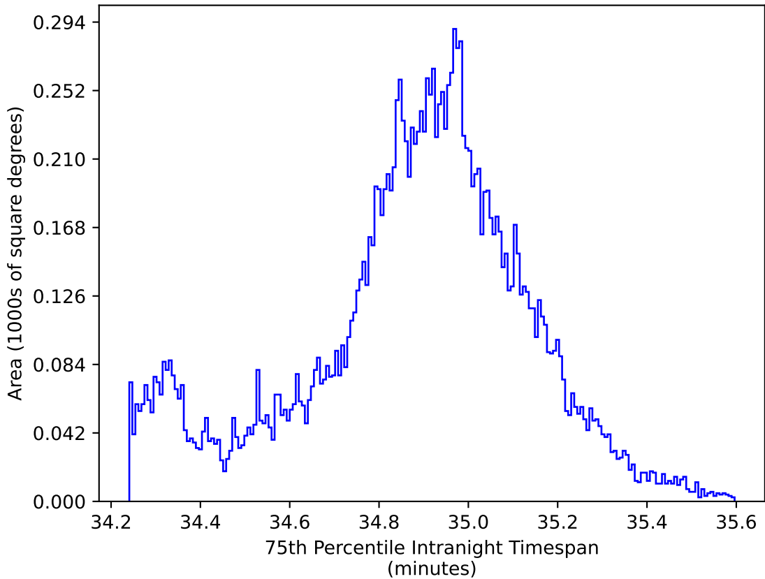
too_elab_r64_d2_griz_v3.4_10yrs WFD: 75th Percentile Intranight Timespan
