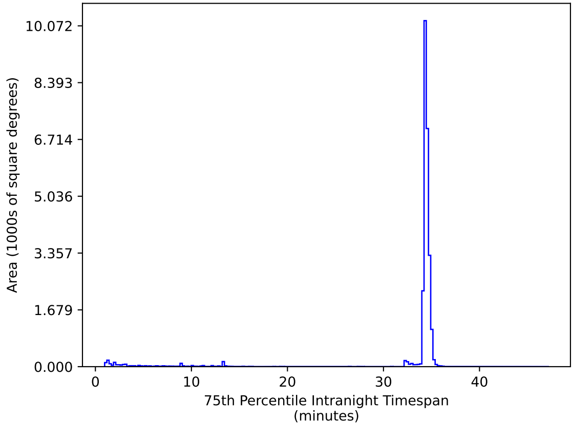
too_elab_r64_d2_griz_v3.4_10yrs All sky zy bands: 75th Percentile Intranight Timespan
