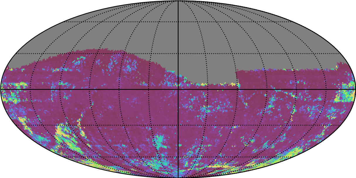
too_elab_r64_d2_griz_v3.4_10yrs All sky z band: 75th Percentile Intranight Timespan
