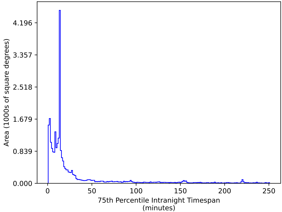
too_elab_r64_d2_griz_v3.4_10yrs All sky z band: 75th Percentile Intranight Timespan
