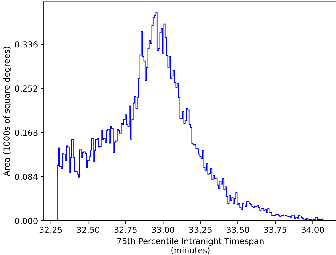
too_elab_r64_d2_griz_v3.4_10yrs All sky y band: 75th Percentile Intranight Timespan
