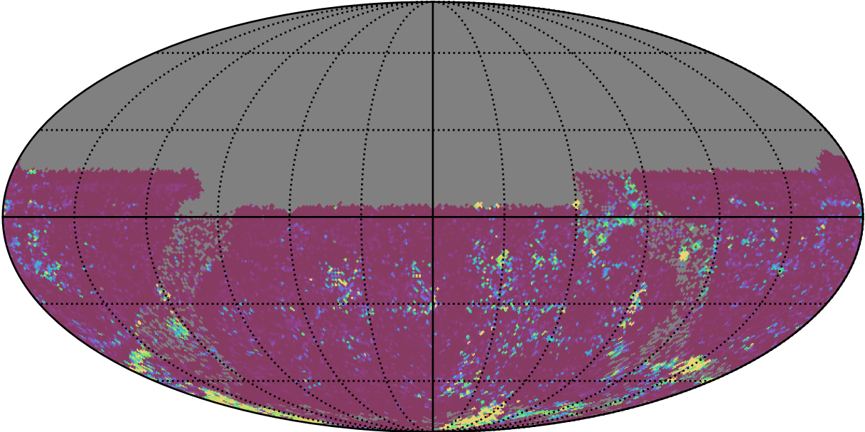
too_elab_r64_d2_griz_v3.4_10yrs All sky u band: 75th Percentile Intranight Timespan
