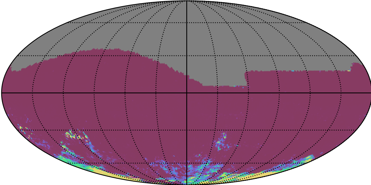
too_elab_r64_d2_griz_v3.4_10yrs All sky ri bands: 75th Percentile Intranight Timespan
