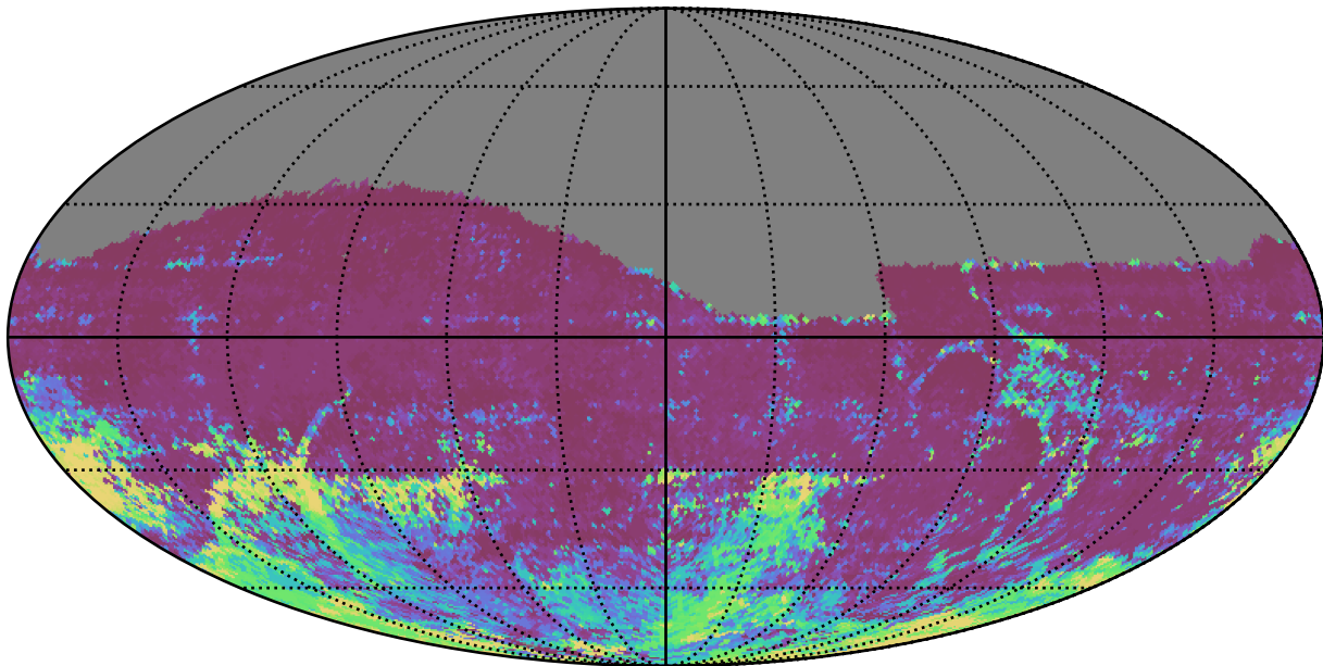
too_elab_r64_d2_griz_v3.4_10yrs All sky r band: 75th Percentile Intranight Timespan
