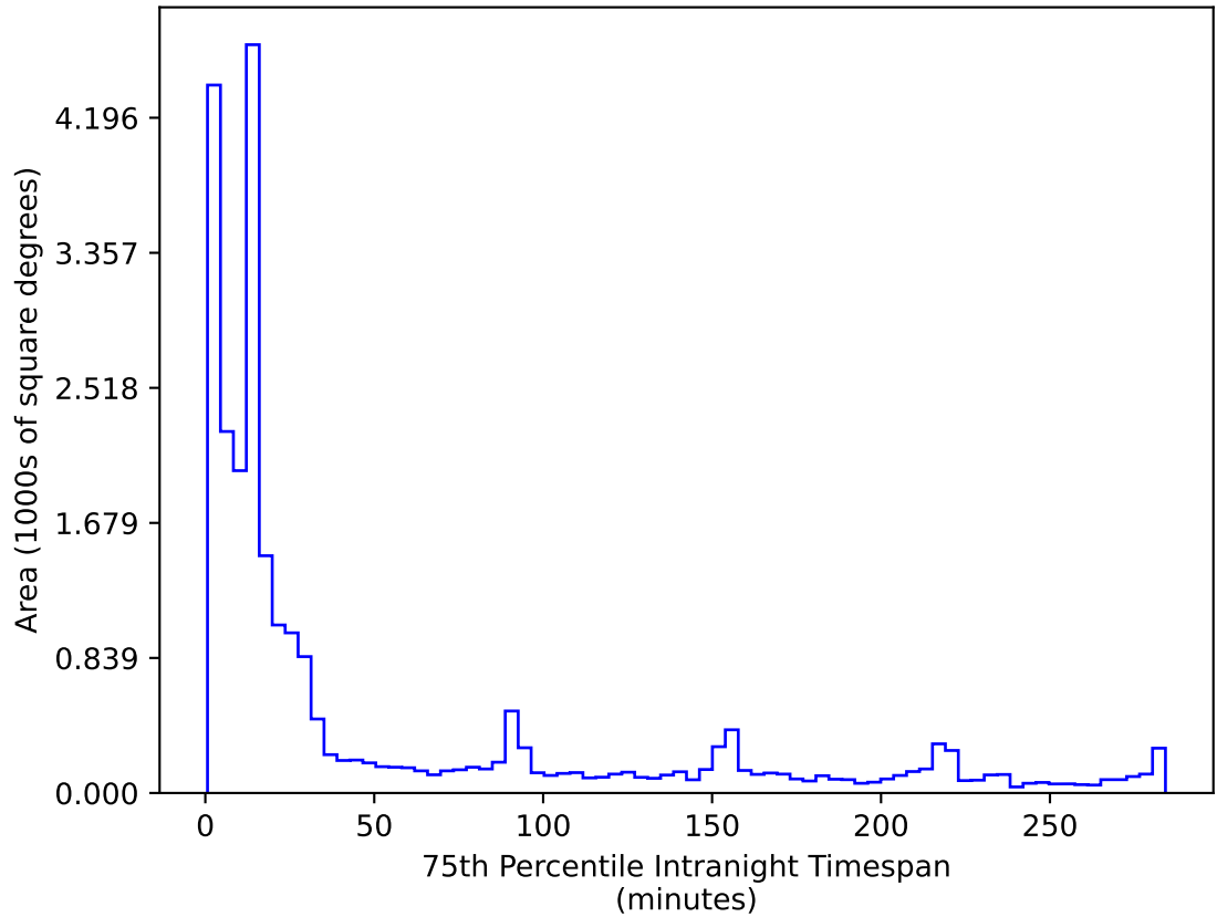
too_elab_r64_d2_griz_v3.4_10yrs All sky r band: 75th Percentile Intranight Timespan
