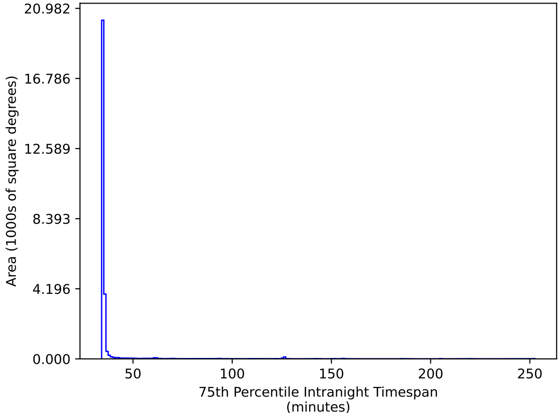
too_elab_r64_d2_griz_v3.4_10yrs All sky gr bands: 75th Percentile Intranight Timespan
