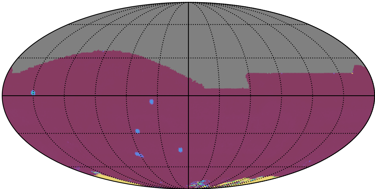
too_elab_r64_d2_griz_v3.4_10yrs All sky: 75th Percentile Intranight Timespan
