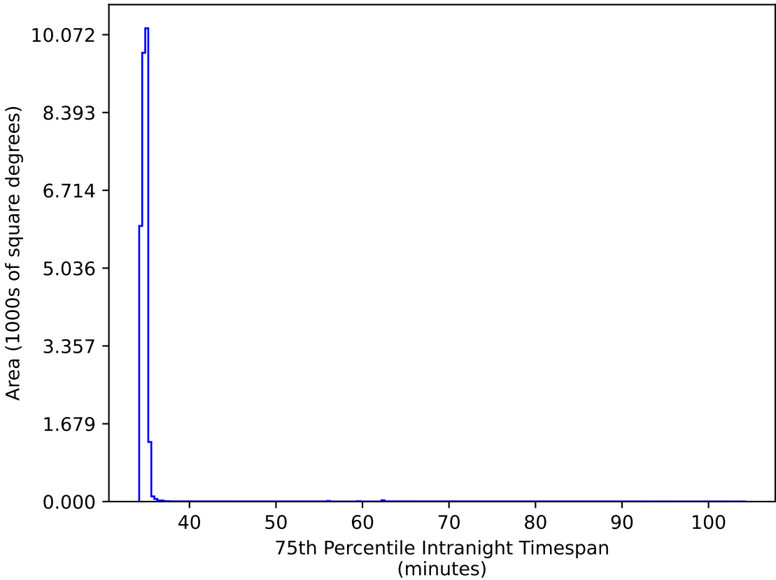
too_elab_r64_d2_griz_v3.4_10yrs All sky: 75th Percentile Intranight Timespan
