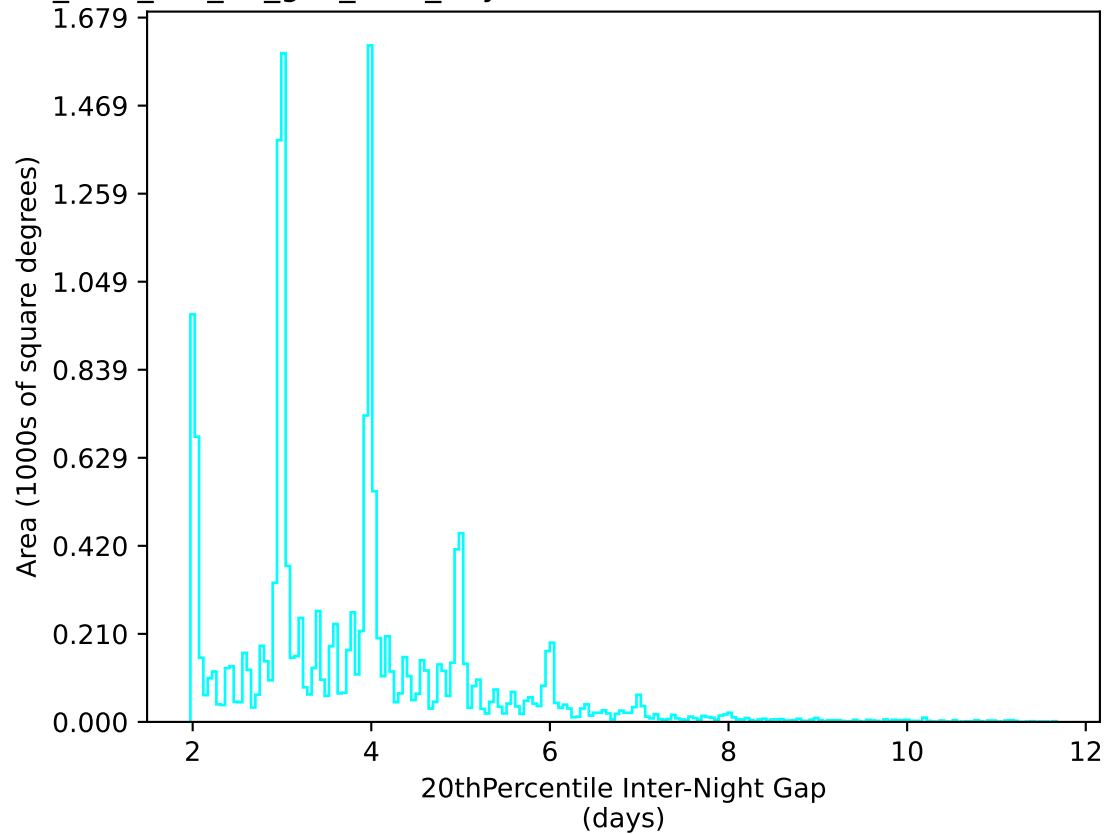
too_elab_r64_d2_griz_v3.4_10yrs WFD u band: 20thPercentile Inter-Night Gap
