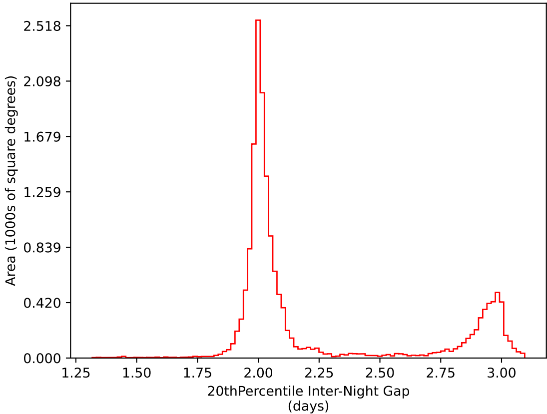
too_elab_r64_d2_griz_v3.4_10yrs WFD i band: 20thPercentile Inter-Night Gap
